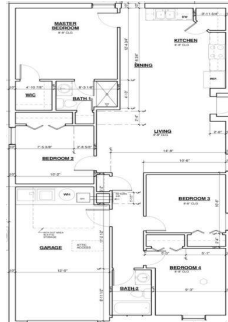
Rent Buster Series Living Area.....1257 sqft. Car Garage....302 sqft. Total.....1619 sqft.
